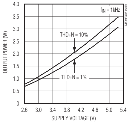
OUTPUT POWER vs. SUPPLY VOLTAGE (MAX98307)
