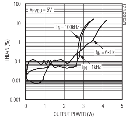
TOTAL HARMONIC DISTORTION PLUS NOISE vs. OUTPUT POWER (MAX98307)
