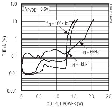
TOTAL HARMONIC DISTORTION PLUS NOISE vs. OUTPUT POWER (MAX98308)
