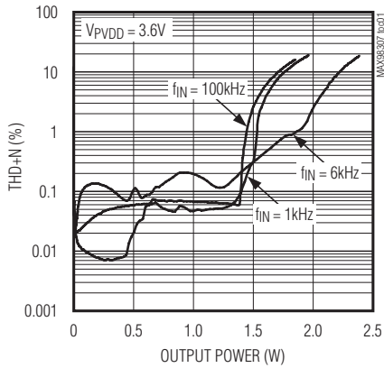
TOTAL HARMONIC DISTORTION PLUS NOISE vs. OUTPUT POWER (MAX98307)
