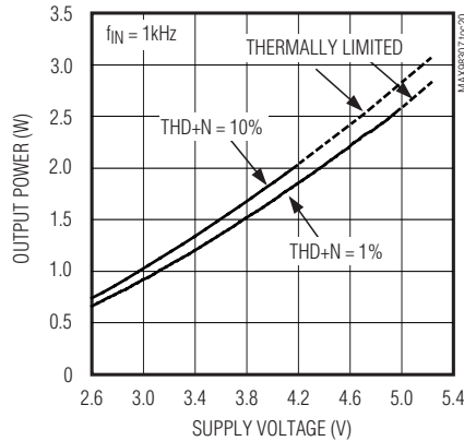
OUTPUT POWER vs. SUPPLY VOLTAGE (MAX98308)
