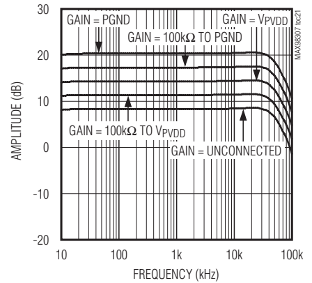
GAIN vs. FREQUENCY (MAX98308)
