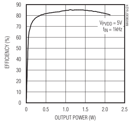
EFFICIENCY vs. OUTPUT POWER (MAX98307)
