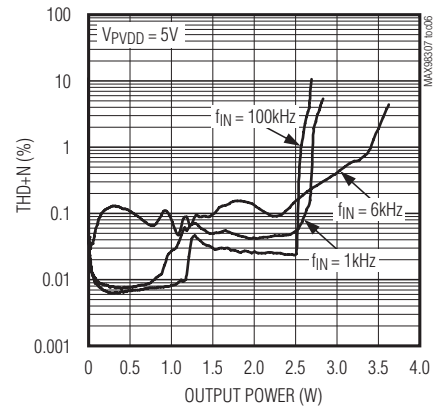
TOTAL HARMONIC DISTORTION PLUS NOISE vs. OUTPUT POWER (MAX98308)
