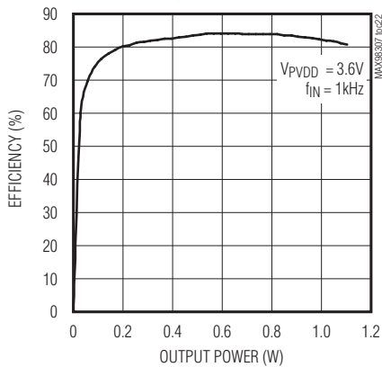
EFFICIENCY vs. OUTPUT POWER (MAX98307)
